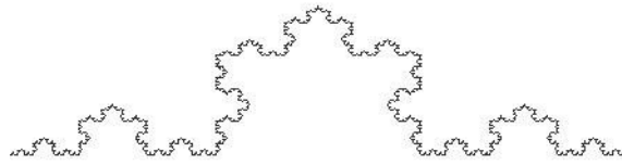
Fig.1 Koch-curve
