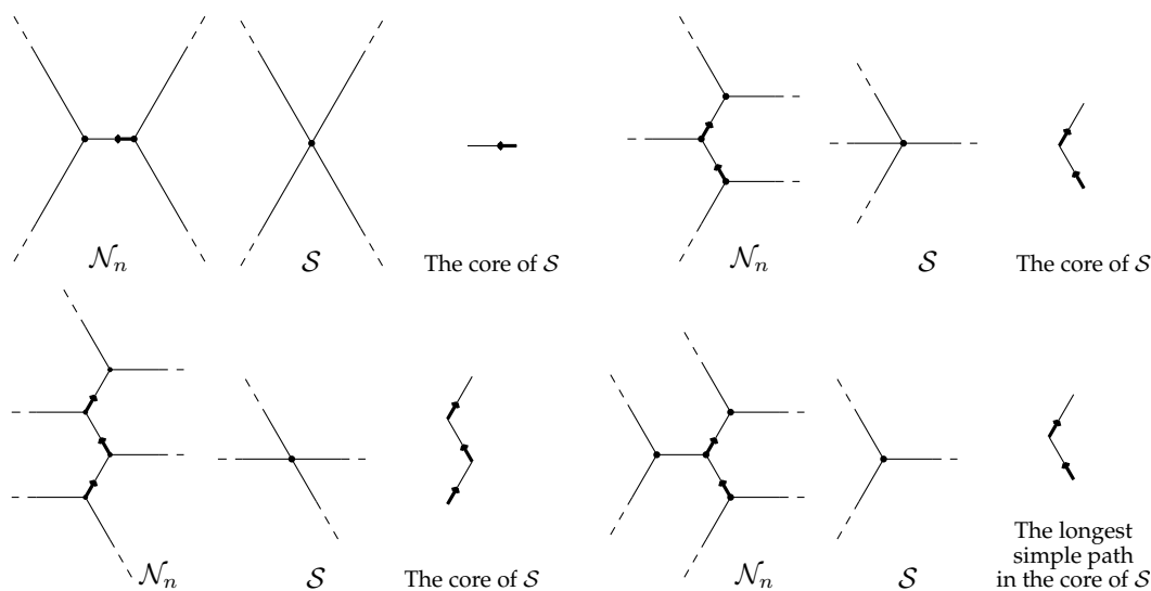
Figure 4: The possible local structure of the graphs G , with relative networks \mathcal{S} and cores, for N = 2, 3, 4 .
