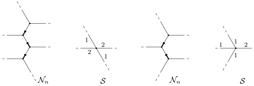
Figure 3: Examples of the edges at the initial/final points of the longest simple path in \mathcal{N}_n and of the relative curves in \mathcal{S} , the numbers 1 and 2 denote their multiplicity.
