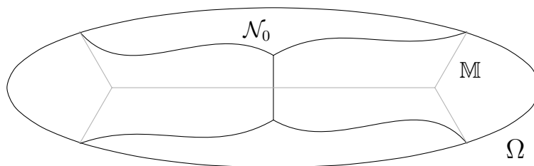
Figure 7: The networks \mathcal{N}_0 and \mathbb{M} .
